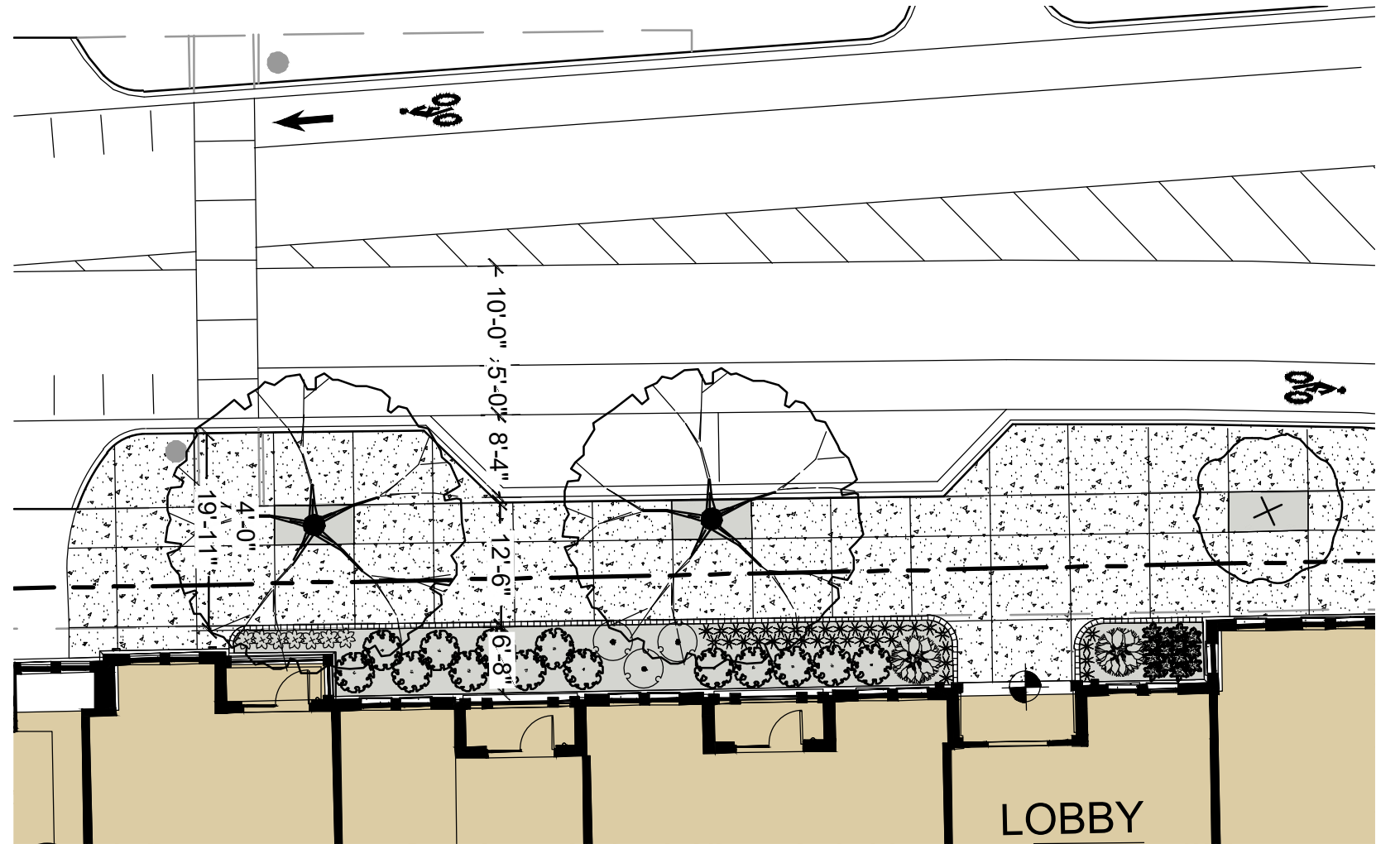
2 BROAD STREET EAST STREETScape PLAN L2 SCALE: 1/16"=1'
