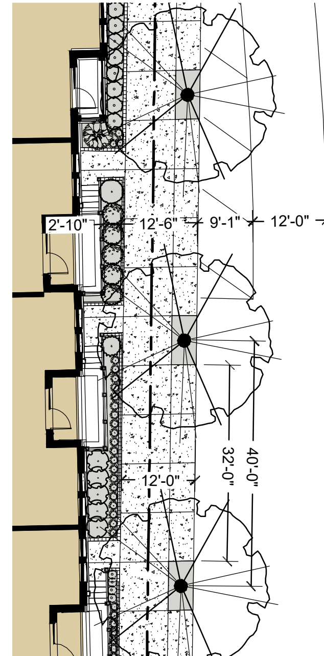
2 SPRING STREET STREETScape PLAN L1 SCALE: 1/16"=1'
