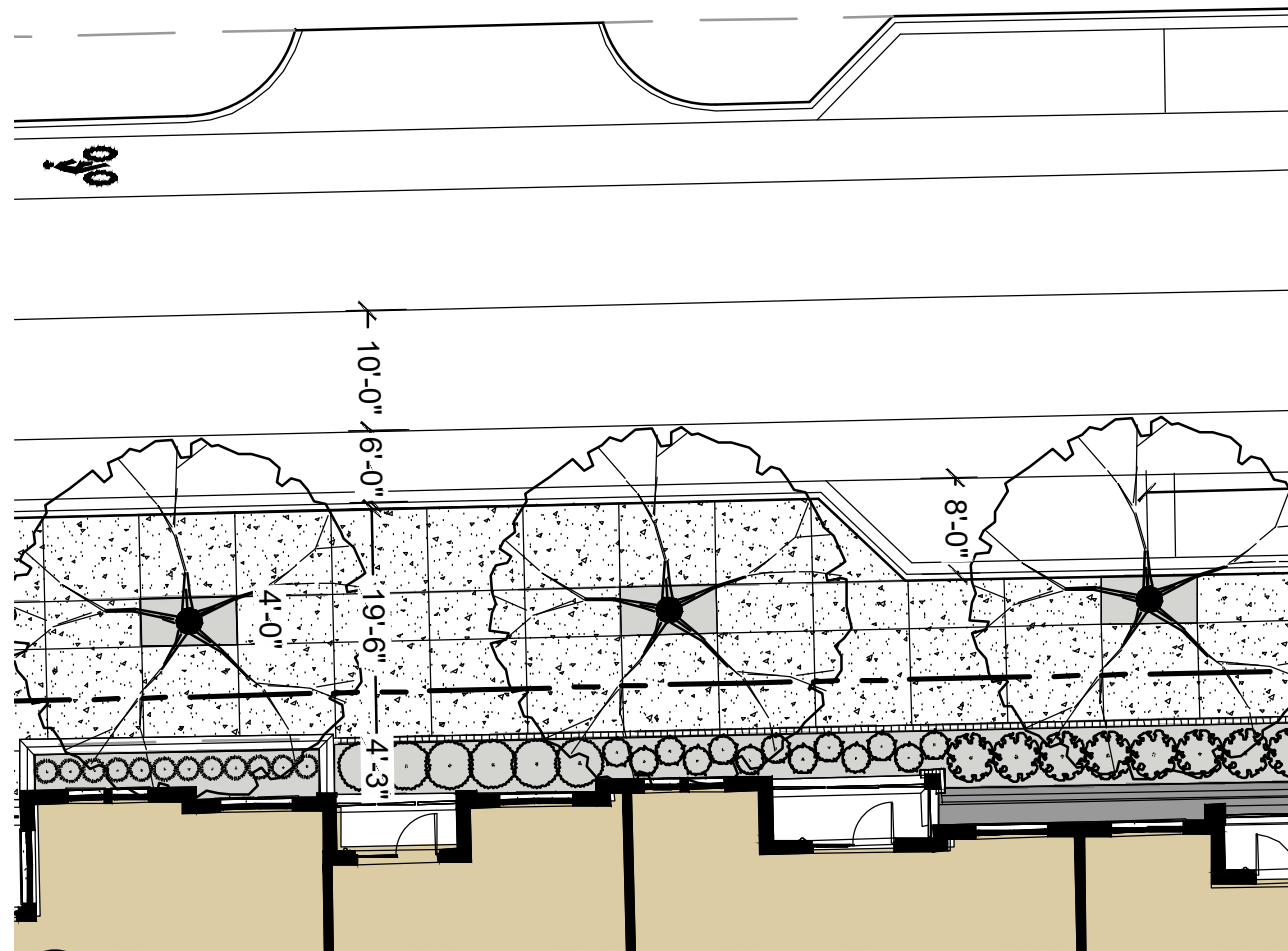
1 BROAD STREET WEST STREETScape PLAN L2 SCALE: 1/16"=1'
